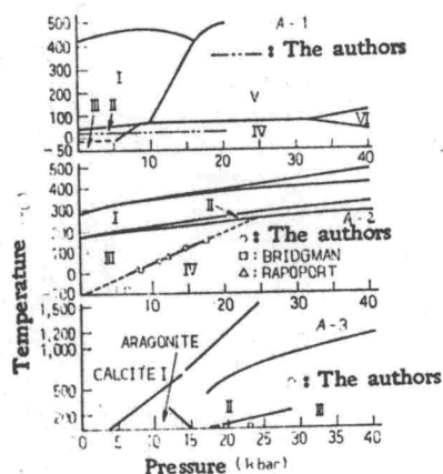
Fig. A1. Temperature-pressure phase diagrams for \text{KNO}_2 (A-1), \text{NaNO}_3 (A-2) and \text{CaCO}_3 (A-3) (after Rapoport).
